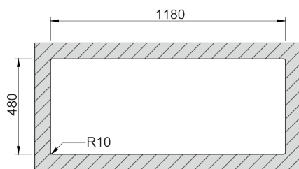
Inset Installation
